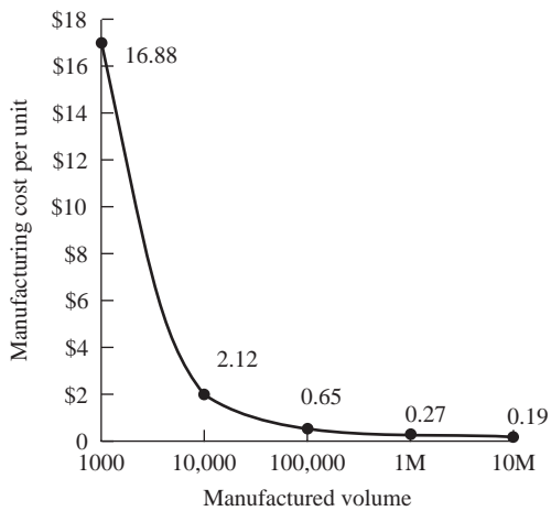
Figure 11.9 The effect of volume on the cost of a plastic part.
