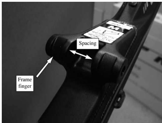
Figure 10.12 Shock-frame connection.
